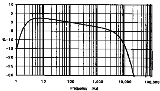
TYPICAL FREQUENCY RESPONSE, MODEL 7250AM2
