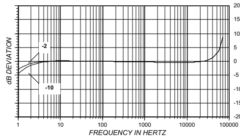
TYPICAL AMPLITUDE RESPONSE, MODEL 7250AM1
