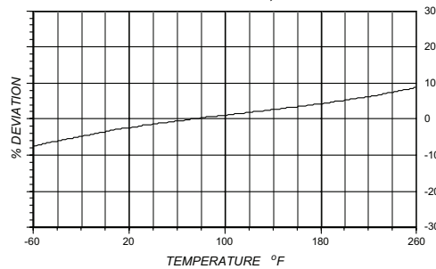
TYPICAL TEMPERATURE RESPONSE, MODEL 7250AM1 / 2
